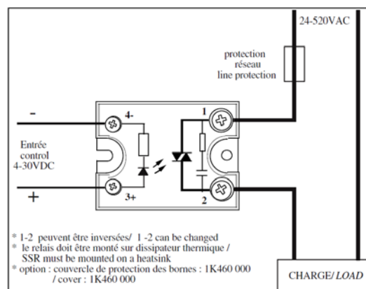
Application typique/Typical application
